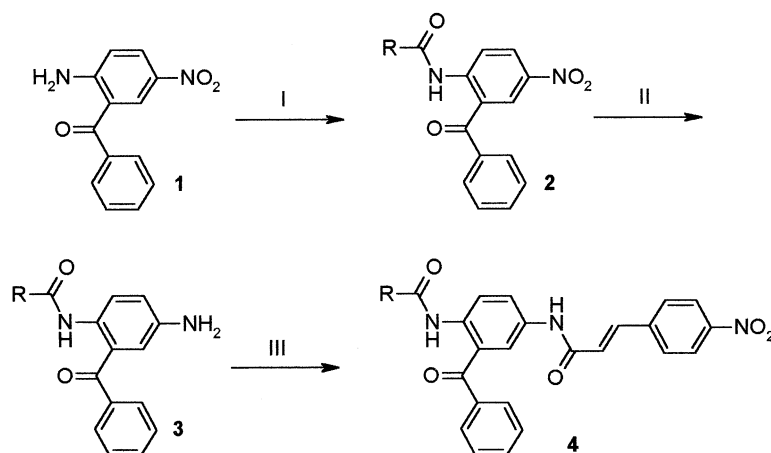
Scheme 1. (i) R–CO–Cl, toluene/dioxane, reflux, 2 h; (ii) SnCl 2 ×2H 2 O, EtOAc, reflux 2 h; (iii) 4-nitrocinnamic acid chloride, toluene/dioxane, reflux, 2 h.
