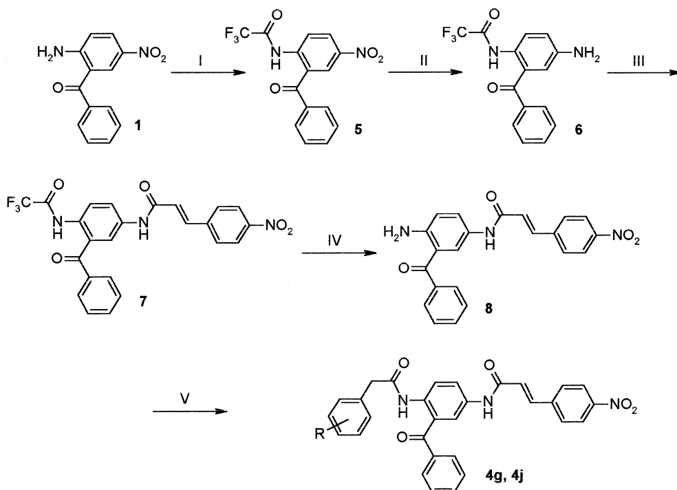
Scheme 2. (i) TFAA, DCM/pyridine, 0 °C, 2 h; (ii) SnCl 2 ×2H 2 O, EtOAc, reflux 2 h; (iii) 4-nitrocinnamic acid chloride, toluene/dioxane, reflux, 2 h; (iv) K 2 CO 3 , dioxane/H 2 O, reflux, 3 h; (v) R–C 6 H 4 –CH 2 –COCl, toluene/dioxane, reflux, 2 h.
